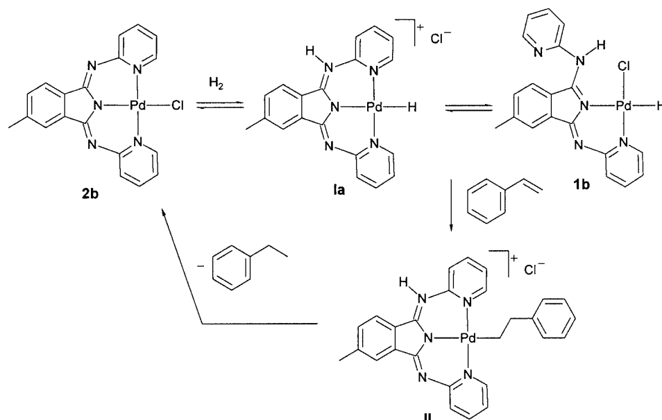
Scheme 4. Proposed mechanism of the Pd-catalyzed hydrogenation
