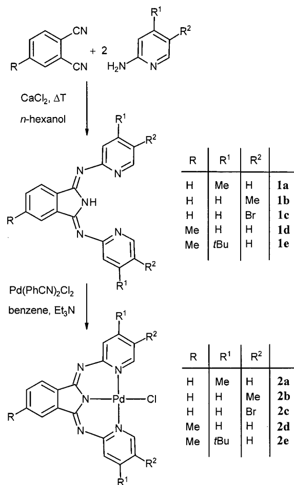
Scheme 1. Synthesis of the BPI-ligands 1a–1e and their palladation to give the Pd II complexes 2a–2e
