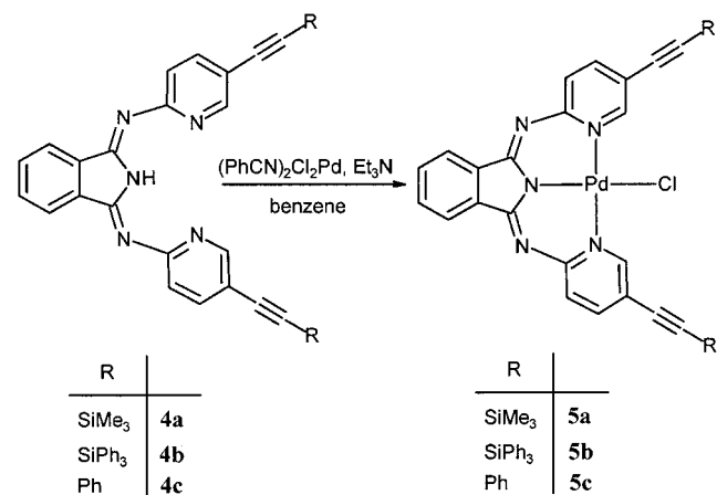
Scheme 3. Synthesis of the alkynyl-substituted BPI-palladium(II) complexes 5a–5c
