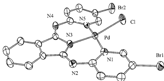
Figure 1. Molecular structure of complex 2c ; selected bond lengths and angles are listed in Table 1
