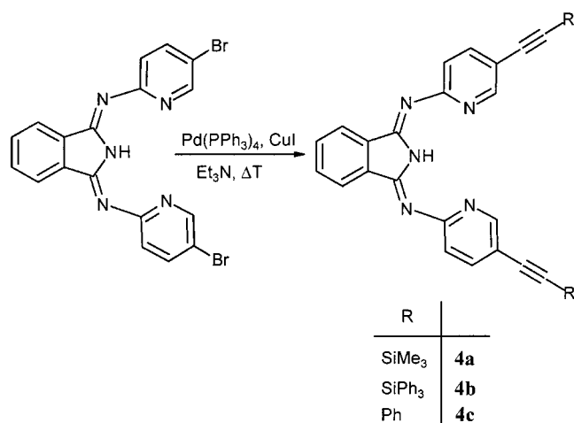
Scheme 2. Synthesis of the alkynyl-substituted BPI ligands 4a–4c
