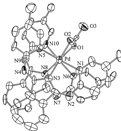
Figure 3. a) Molecular structure of complex 3 ; selected bond lengths (Å) and angles (°): Pd1–N1 2.05(1), Pd2–N6 2.07(1), C41–O1 1.23(2), Pd1–N3 1.93(2), Pd2–N8 1.94(1), C41–O2 1.34(2), Pd1–N5 2.05(1), Pd2–N10 2.06(2), C41–O3 1.22(2), Pd1–O2 2.04(1), Pd2–O1 2.03(1); N1–Pd1–N5 172.5(5), N1–Pd1–O2 89.7(6), N6–Pd2–O1 90.4(7), N6–Pd2–N10 73.4(5), N3–Pd1–O2 178.3(5), N8–Pd2–O1 175.7(6); b) view along the Pd–Pd axis
