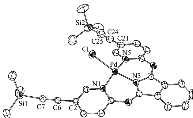
Figure 4. Molecular structure of complex 5a ; selected bond lengths and angles are listed in Table 2
