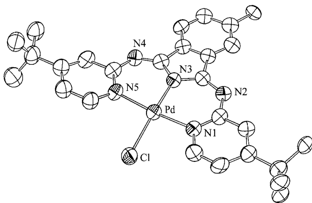
Figure 2. Molecular structure of complex 2e ; selected bond lengths and angles are listed in Table 1
