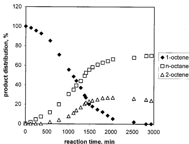
Figure 8. Hydrogenation of 1-octene catalyzed by 2b and the concomitant isomerization of the alkene to a mixture of E - and Z -2-octene, as followed by GC-MS
