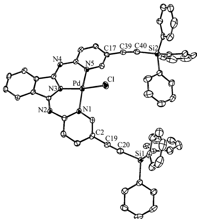
Figure 5. Molecular structure of complex 5b ; selected bond lengths and angles are listed in Table 2
