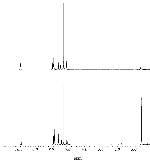
Figure 7. Top: ^1\text{H} NMR spectrum of 2b before the catalysis; bottom: ^1\text{H} NMR spectrum of the catalyst recorded after three cycles of catalysis, isolation of the catalyst, and re-use of the catalyst
