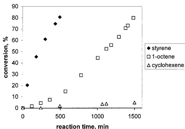
Figure 9. A comparison of the conversion curves for the hydrogenation of styrene, 1-octene and cyclohexene
