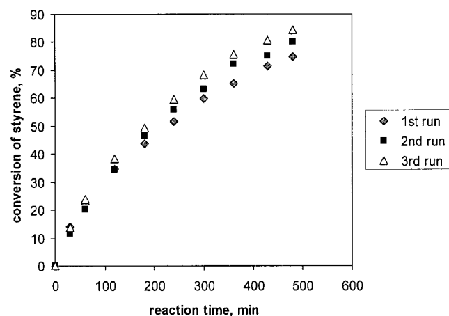
Figure 6. Hydrogenation of styrene at 25 \pm 1 °C in THF at a hydrogen pressure of 1 bar using 2 mol % of the catalyst 2b : a) the conversion curves for three independent catalytic runs; b) isolation of the catalyst that had been used in the third run and re-used in two further catalytic runs
